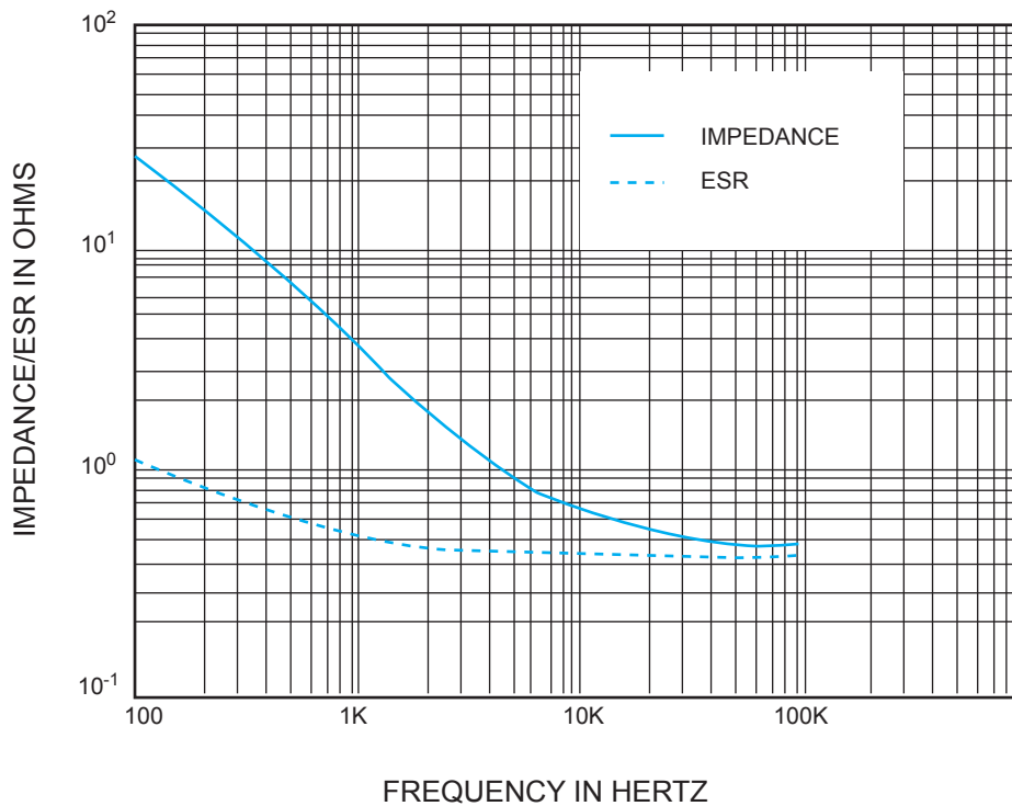
CD266 200V 47 \mu F \Phi 12.5X25
