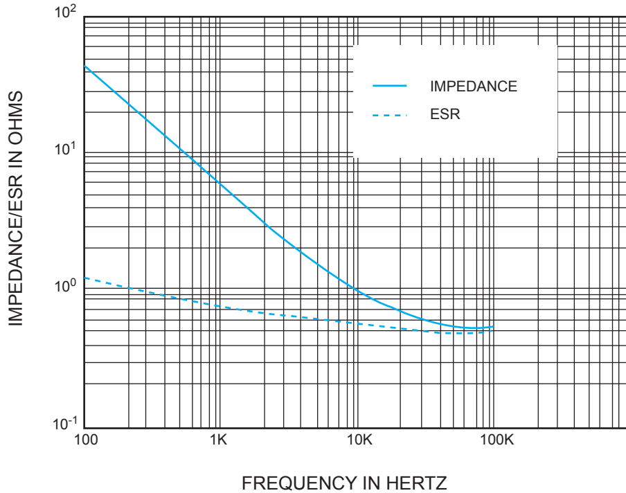
CD266 450V 33 \mu F \Phi 18X35.5
